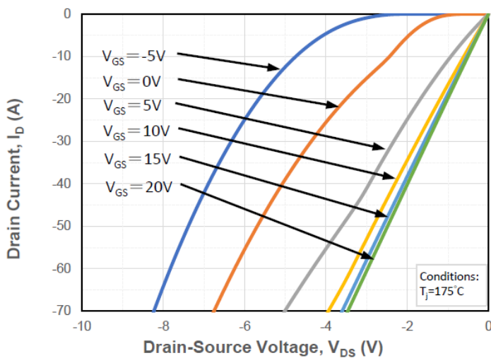
Figure 9. Reverse Output Characteristics at T_j = 175^\circ C
