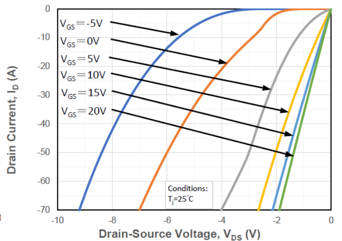
Figure 8. Reverse Output Characteristics at T_j = 25^\circ C
