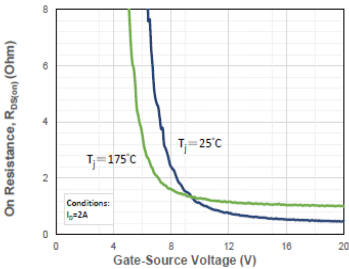
Figure 5. On-resistance vs. gate voltage for various Tj
