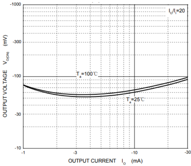
Fig 3: Output Voltage (On) Characteristics
